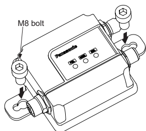
Using M8 bolts for installation (Use larger holes located toward the inside)
