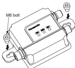
Using M6 bolts for installation (Use smaller holes located toward the outside)
