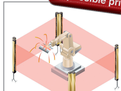
Guarding space around welding robot
